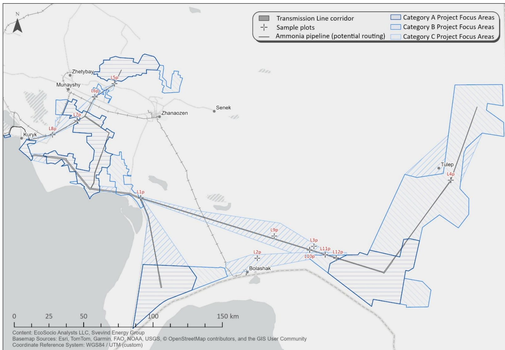
Figure 19: Location of 12 vegetation assessment plots in the transmission line corridors where vegetation was deemed to be more sensitive to the expected impact
