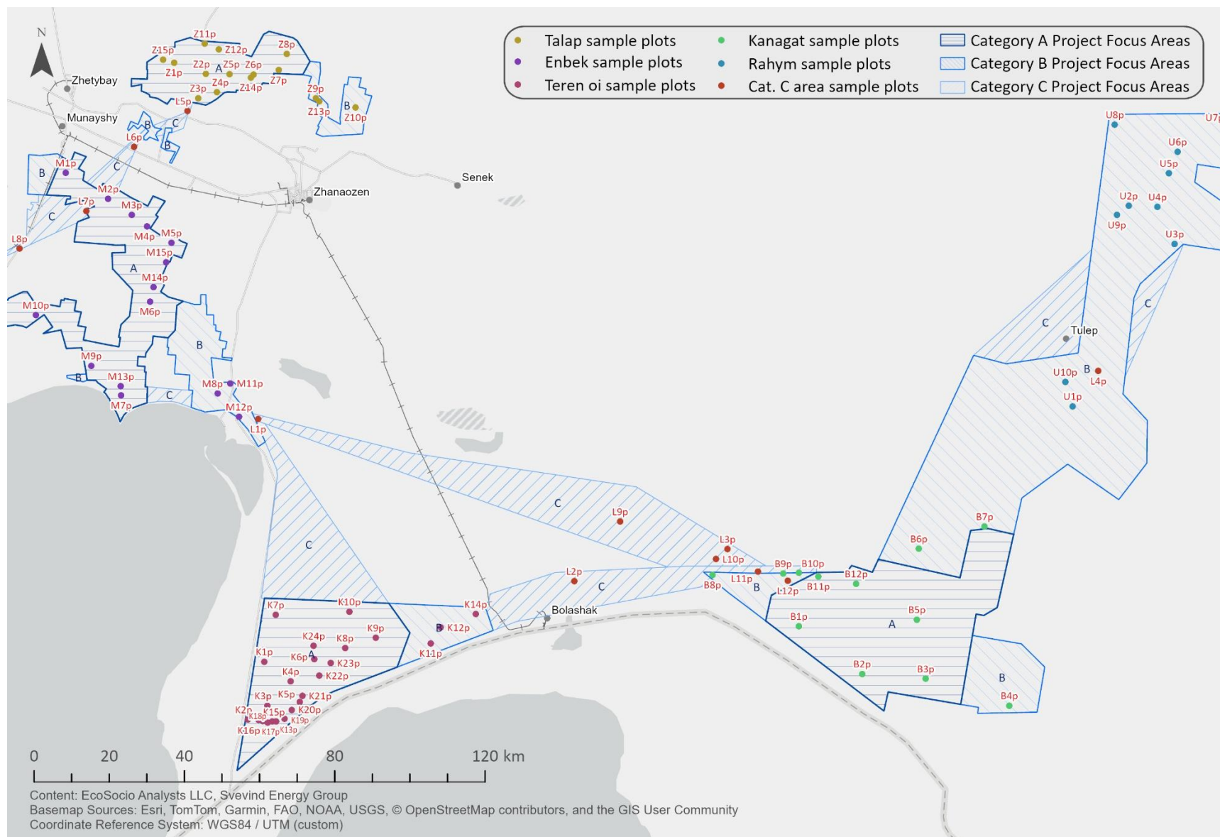
Figure 4: Overview of the flora survey area at renewable energy clusters (Category A and B areas) and overhead transmission line corridors (Category C areas)
