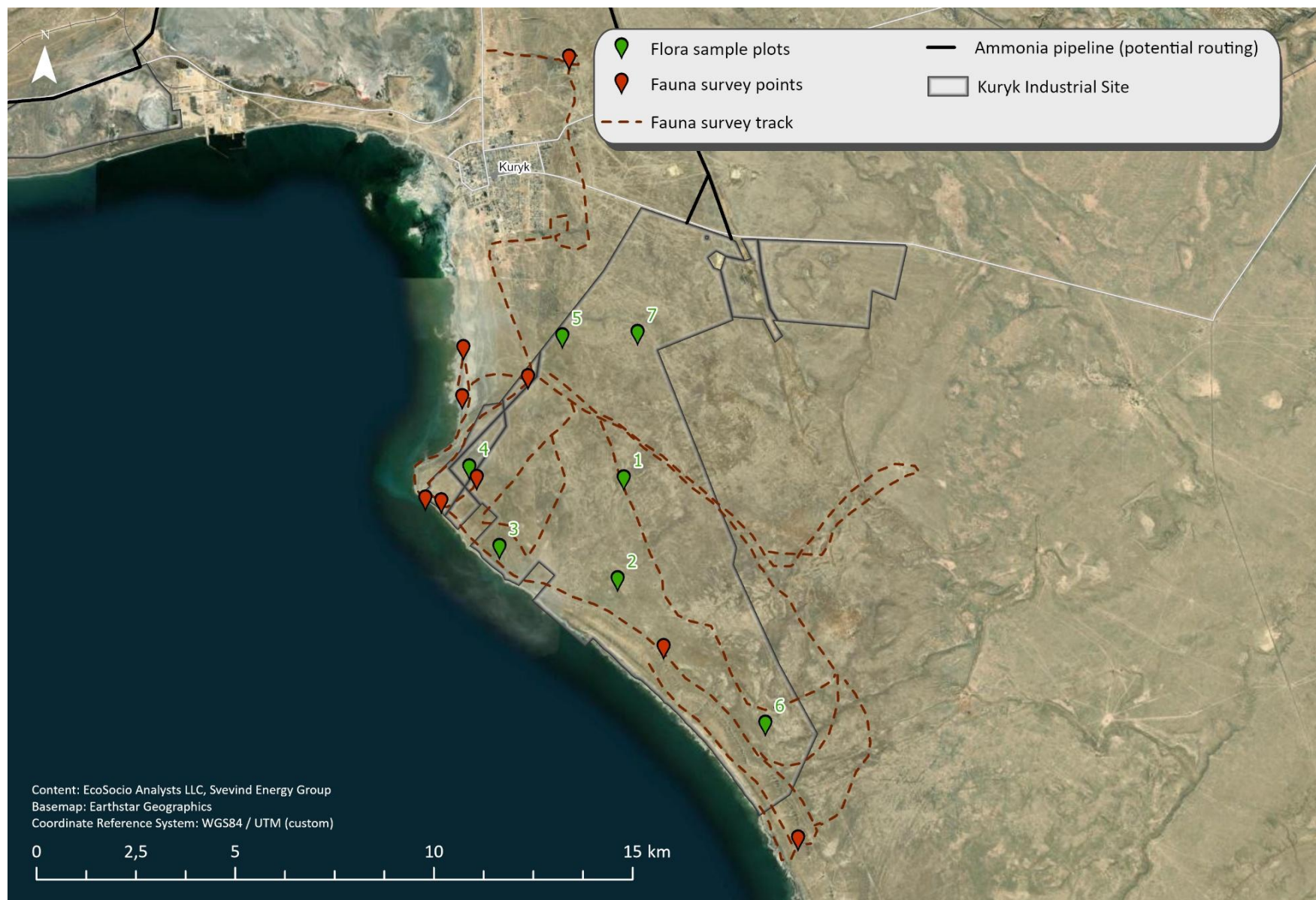
Figure 7: Flora and fauna survey areas at Kuryk Area
