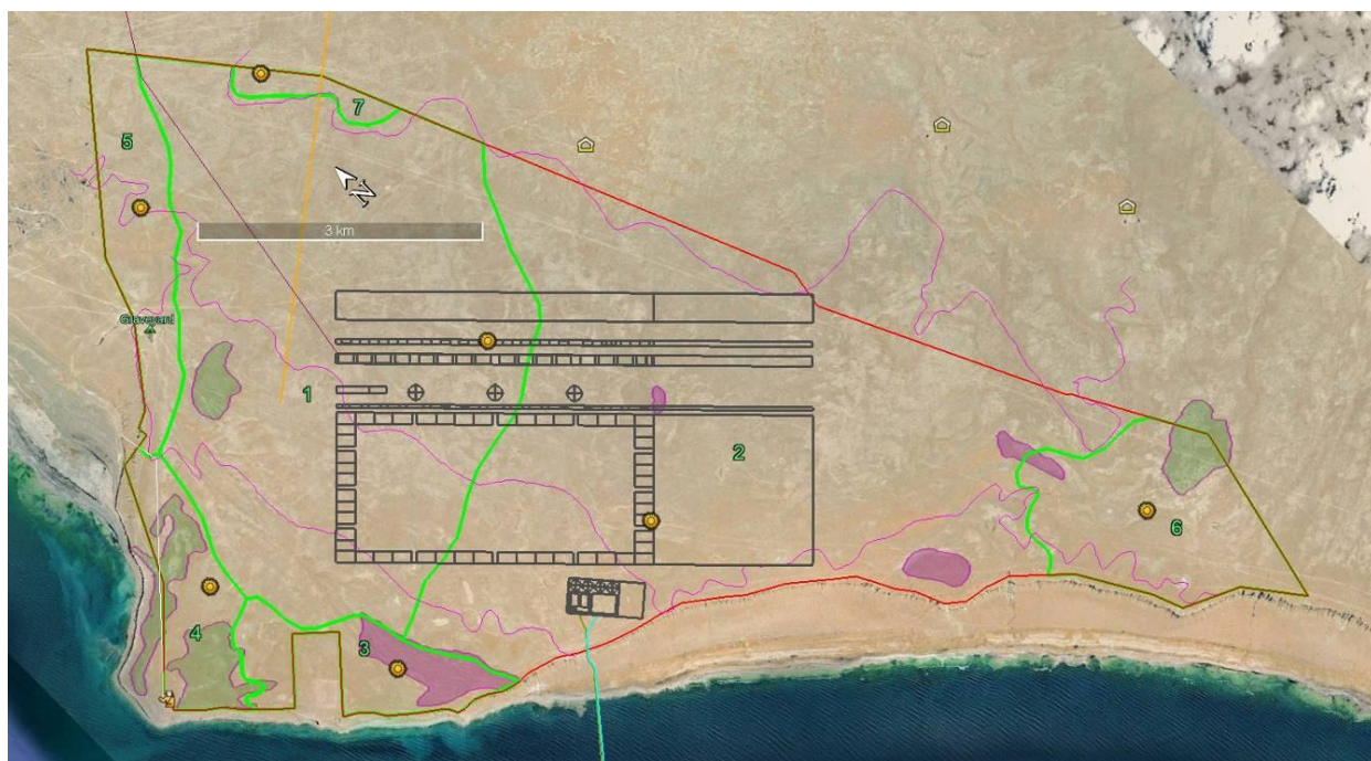
Figure 20: Kuryk area vegetation map with location of 7 plots (yellow) where typical vegetation was described, relief contours 10, 15, 20 and 30 m from the cliff to the east (depressions in green, elevations in purple), and distribution of plant communities (green outline)
